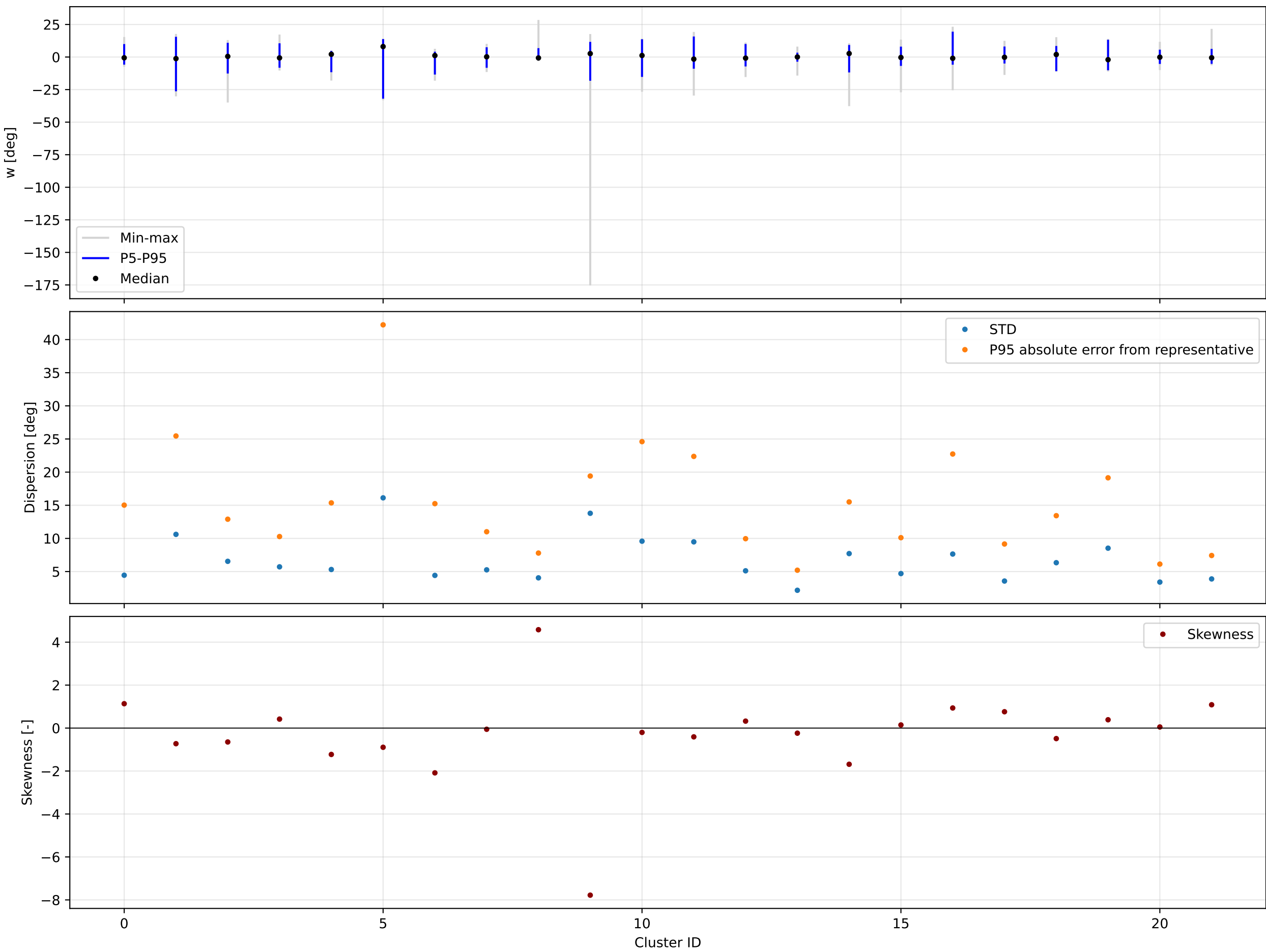
K=22 | backward | w | valid=194058/194058 | offsets from each cluster circular mean
