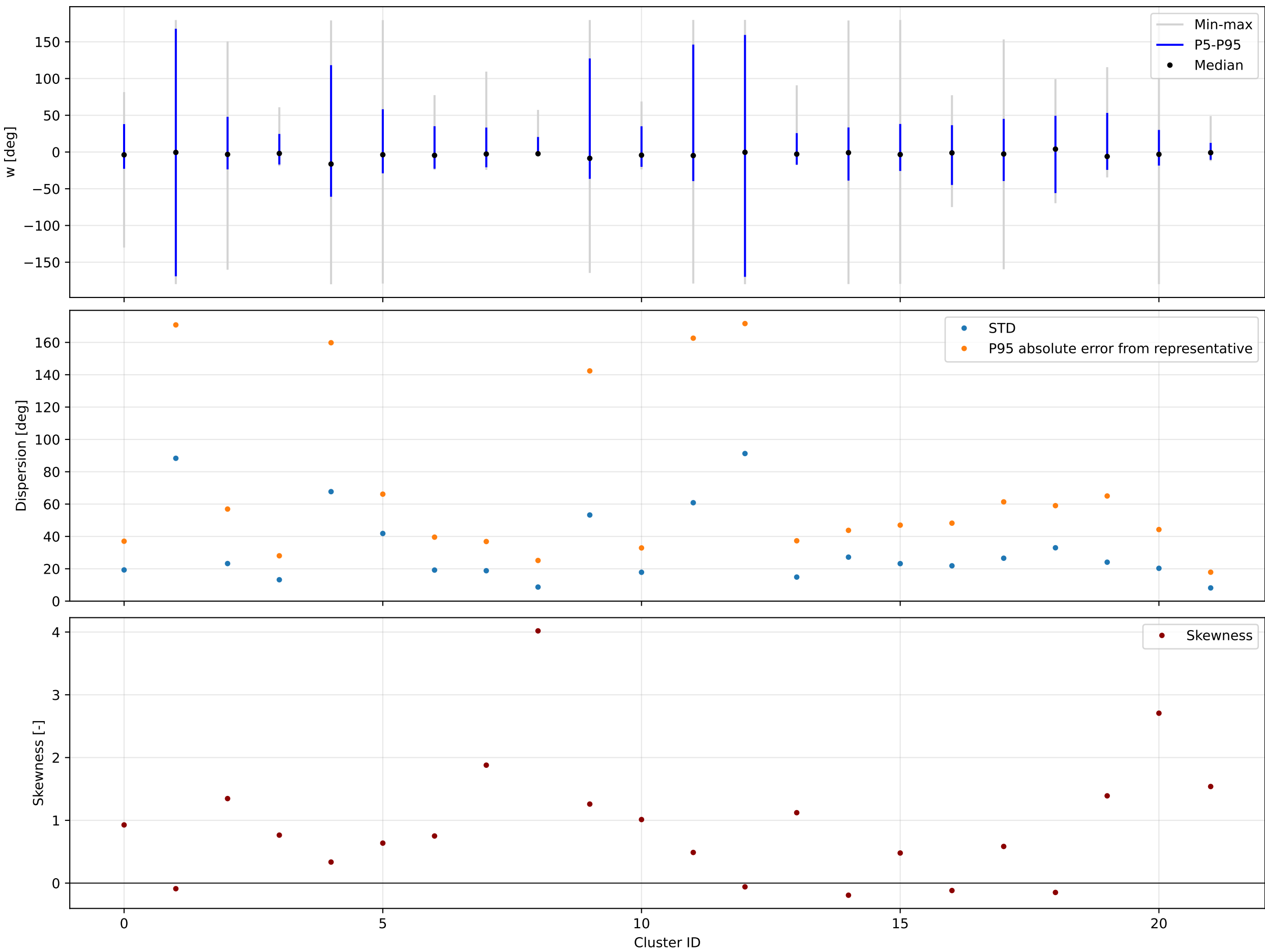
K=22 | forward | w | valid=194058/194058 | offsets from each cluster circular mean
