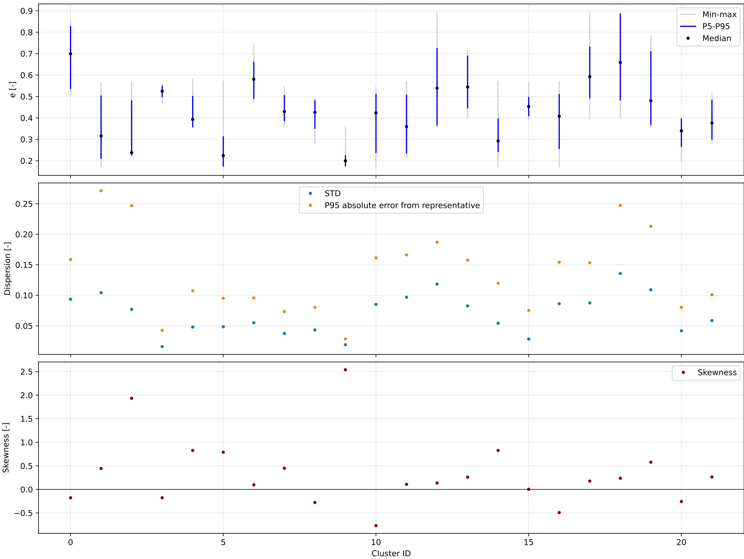
K=22 | backward | e | valid=194058/194058
